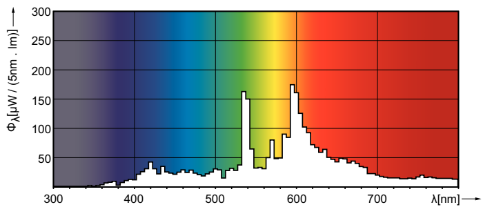
LDPO_CDM-TD_830-Spectral power distribution Colour
