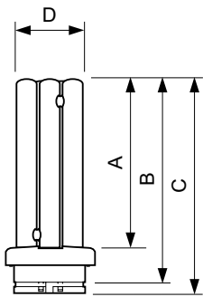
PL-R 17W/840/4P
