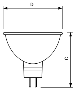
MLES 18144 45W GU5.3 12V MR16 36D
