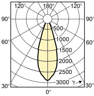
Halogen Reflector 45W GU5.3 12V 36D
