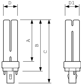
PL-C 26W/840/2P
