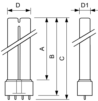
PL-L 36W/840/4P
