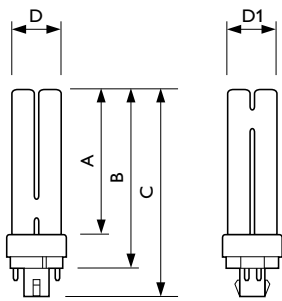
PL-C Xtra 18W/840/4P
