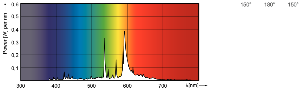
LDPO_CPO-TW_45W_628-Spectral power distribution Colour
