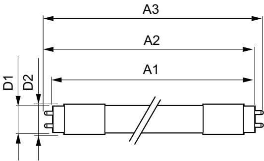
TLED 1200mm 18W865 C
